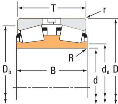
M282249D Bearing 2D drawings and 3D CAD models
